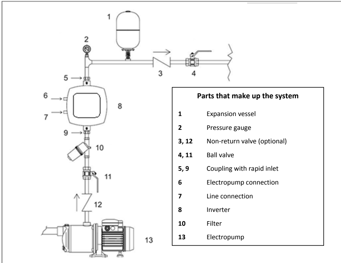
Figure 1: Hydraulic installation
