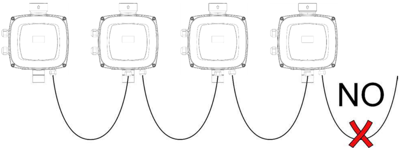
Figure 7: Do not leave cable connected at only one end
