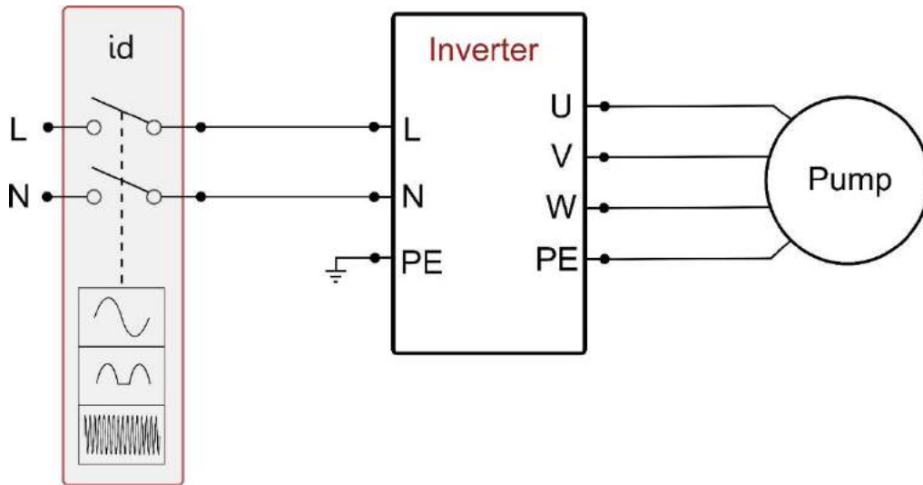
Figure 1a: Example of installation with single-phase power supply
