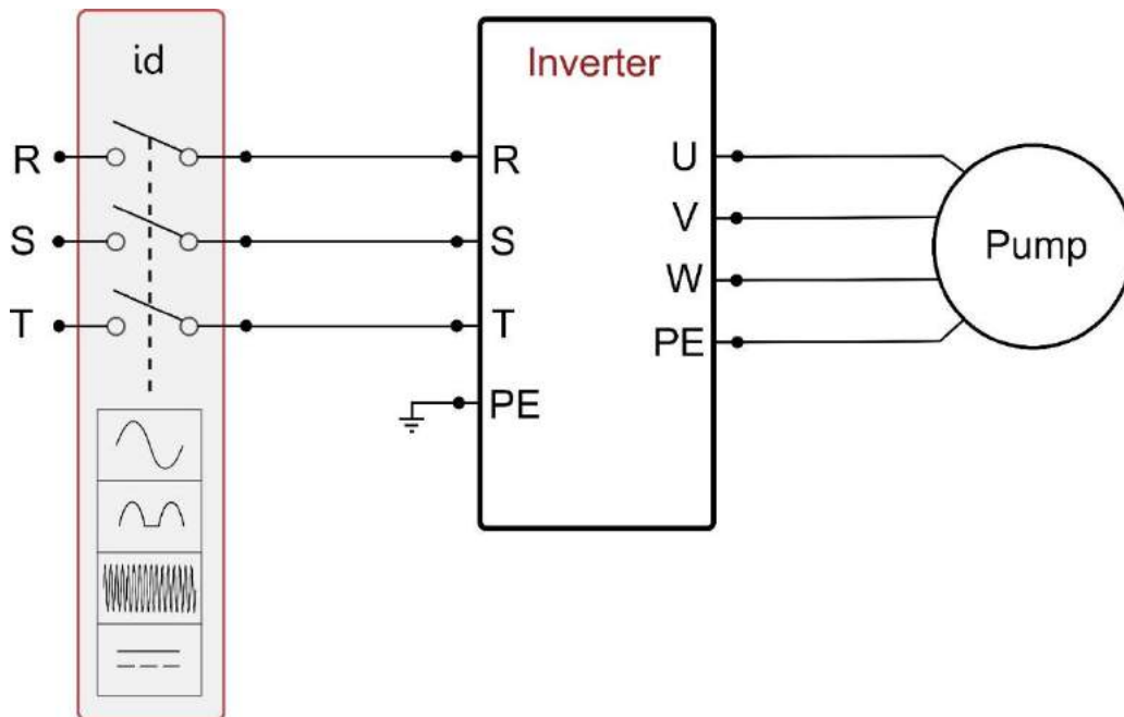
Figure 1b: Example of installation with three-phase power supply
