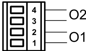
Figure 3: Output connection
