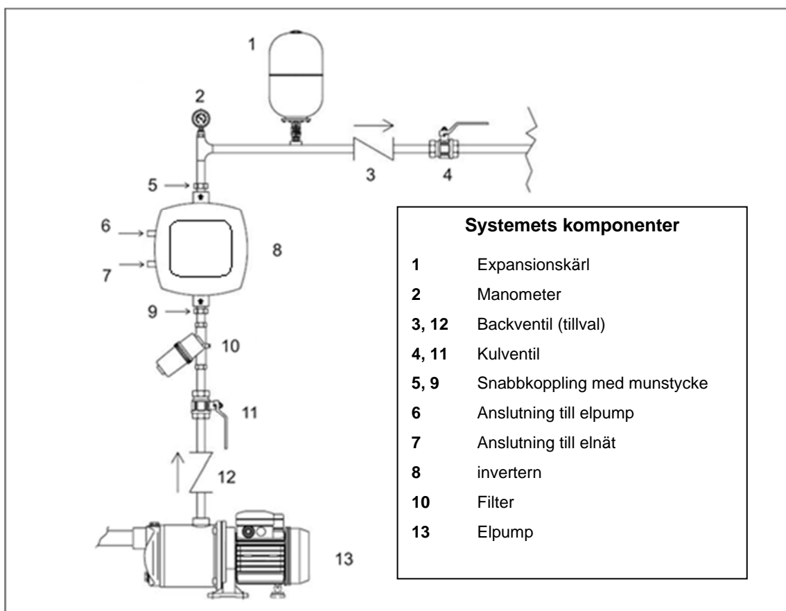
Fig. 1: Hydraulisk installation
