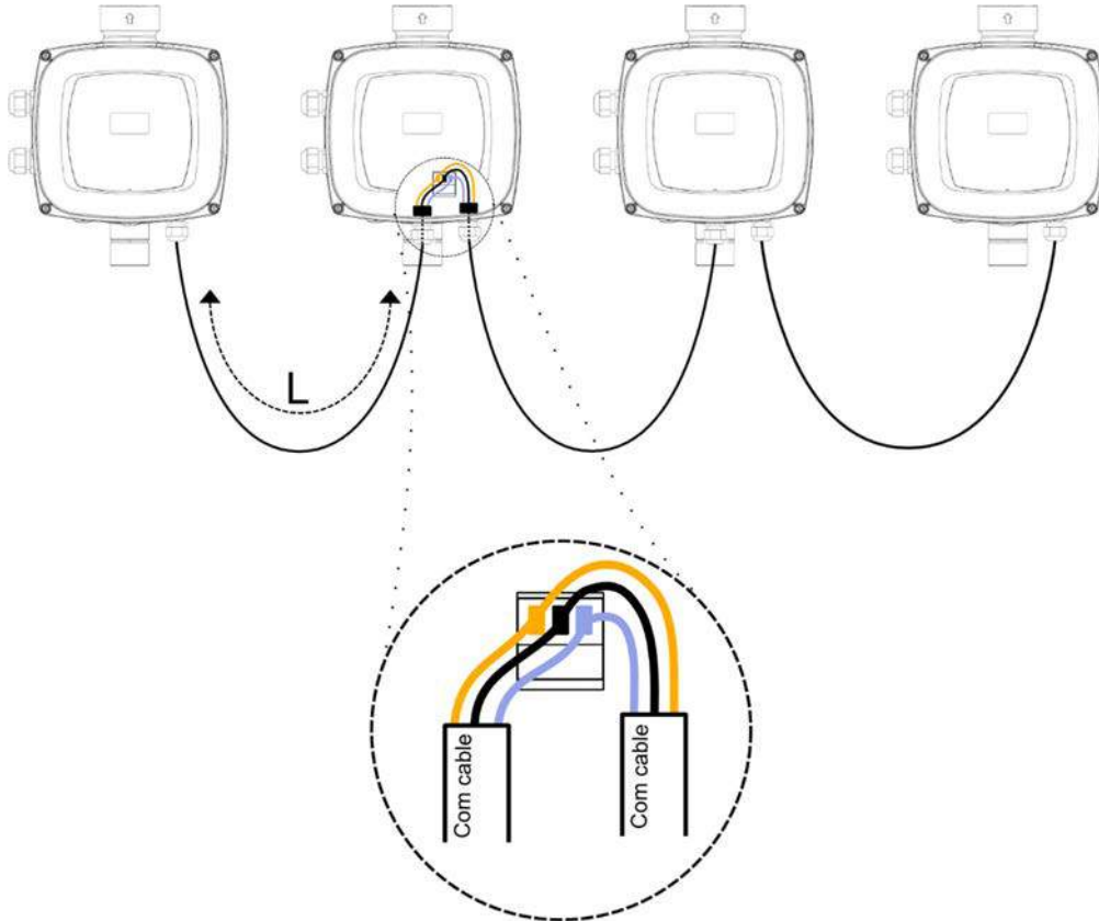
Figure 4: Example of connection of the multi-inverter communication with 4 devices
