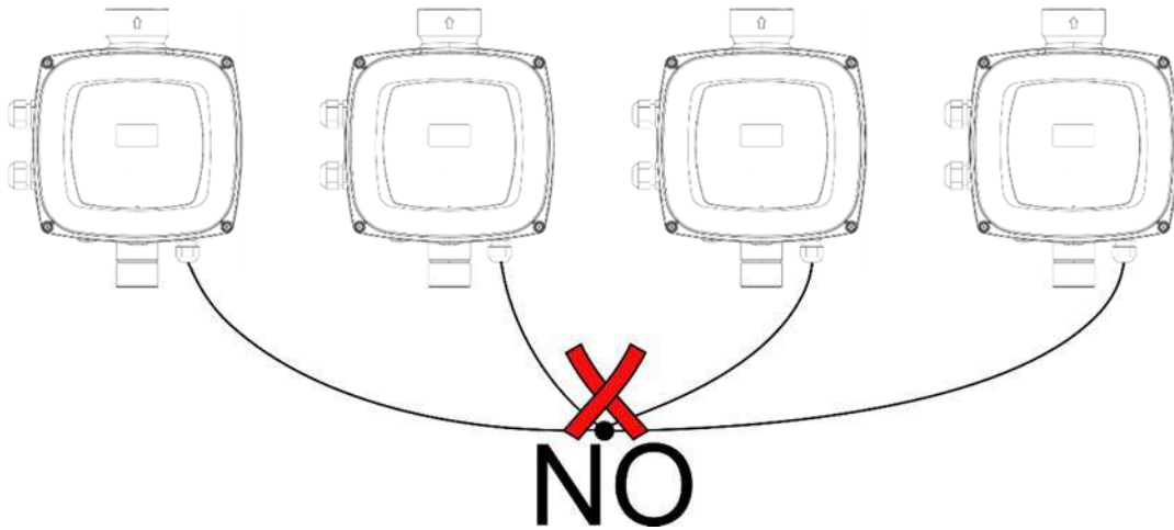
Figure 6: Do not make star connections
