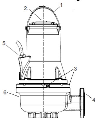
Abb. 1 FK- Pumpe
