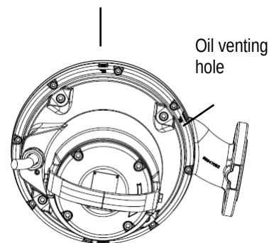
Fig. 11 Oil filling holes
