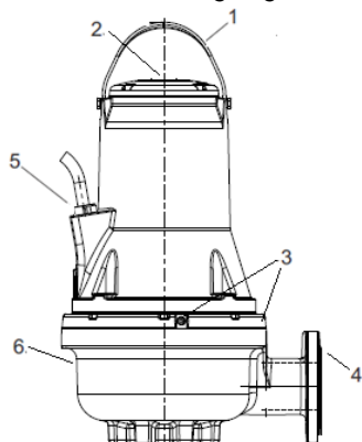
Fig. 1 FK-pumpe
