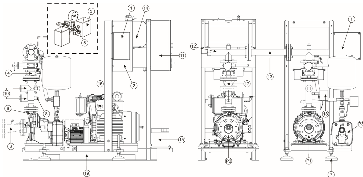
Electrobomba Principal
