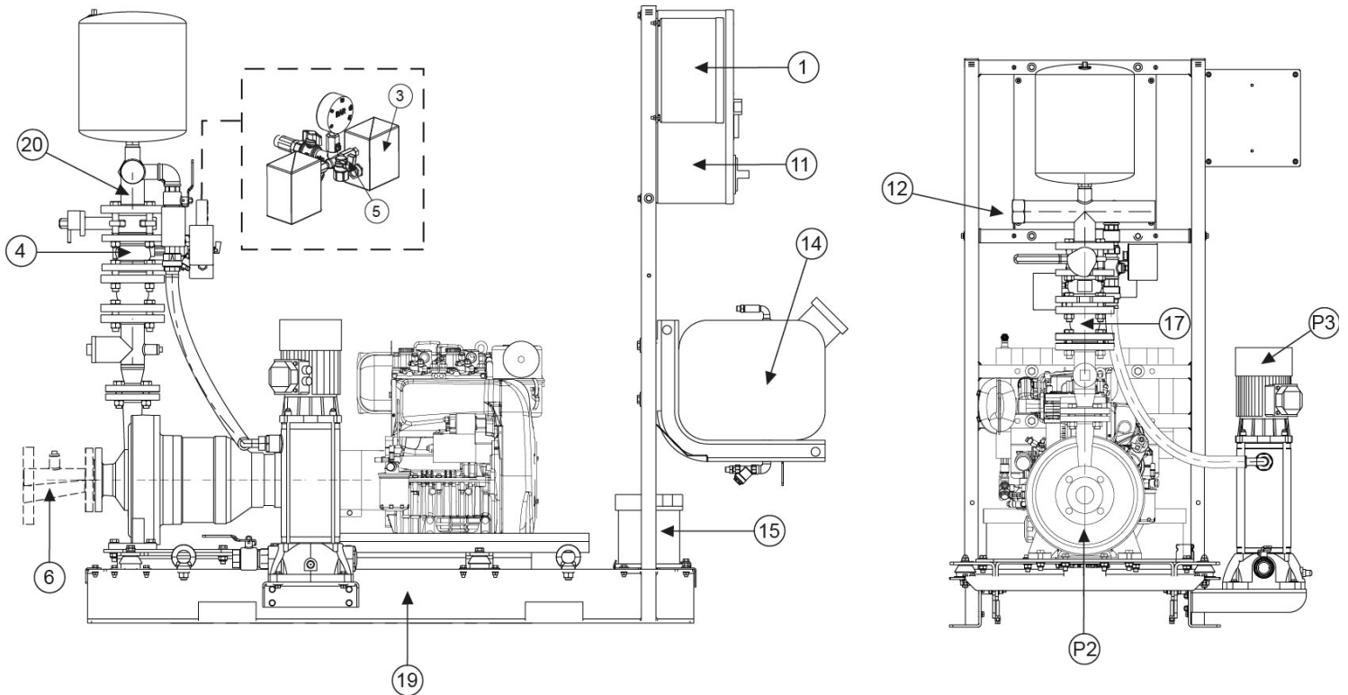
Electrobomba Principal
