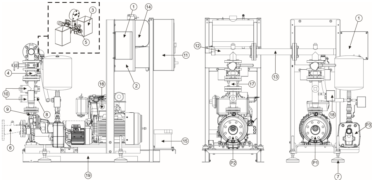
Main Electropump
