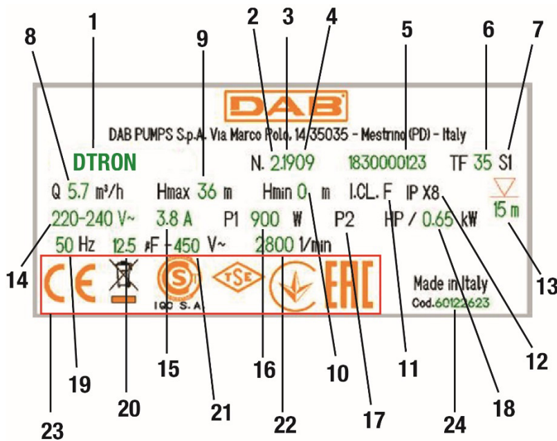
Data plate
