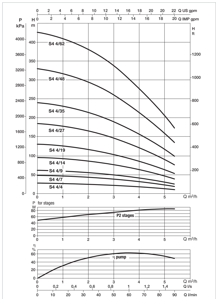
Performance at 50 Hz 2 poles. The performance curves are based on kinematic viscosity values = 1 mm²/s and density equal to 1000 kg/m³. Curve tolerance according to ISO 9906.
