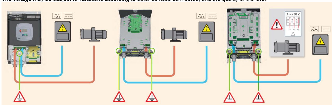
Figure 6: Electrical connections
