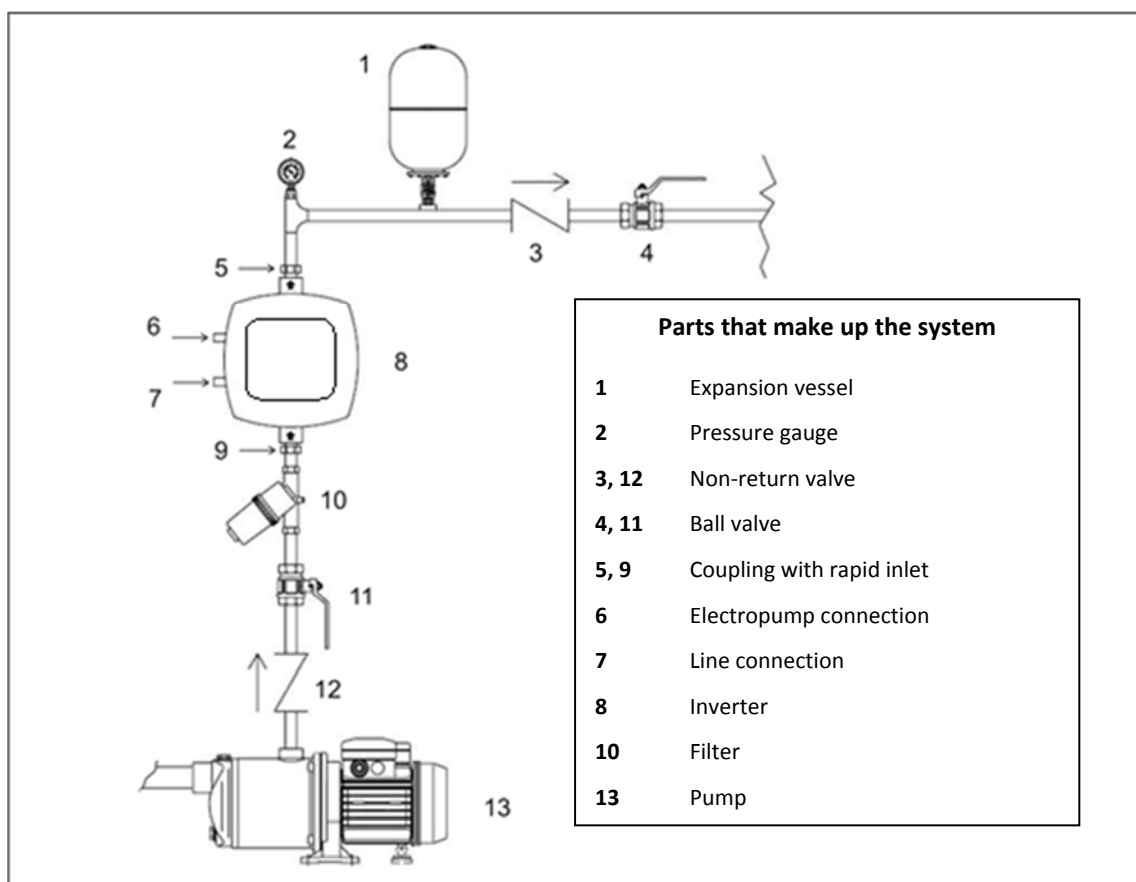
Figure 1: Hydraulic installation
