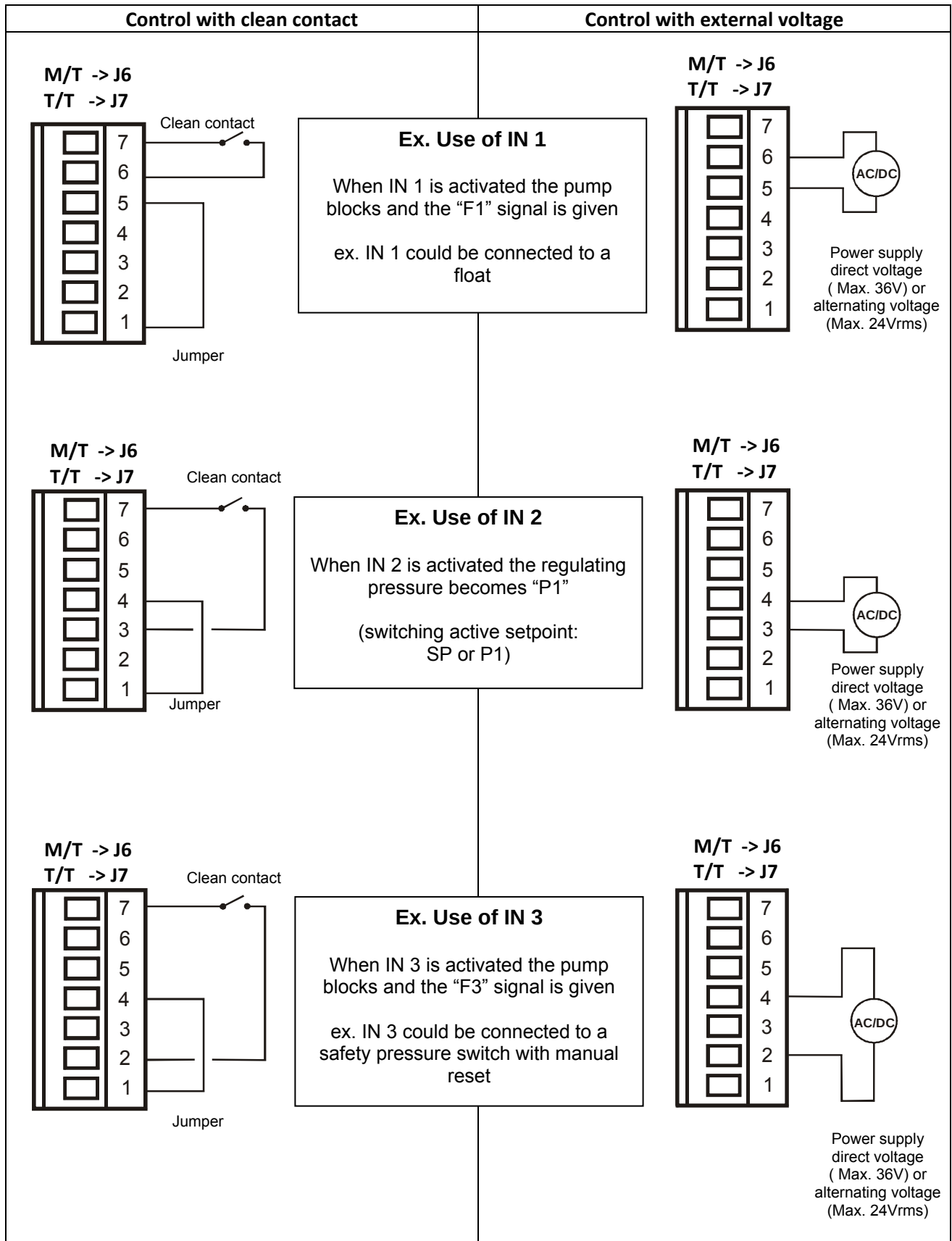
Figure 2: Input connection
