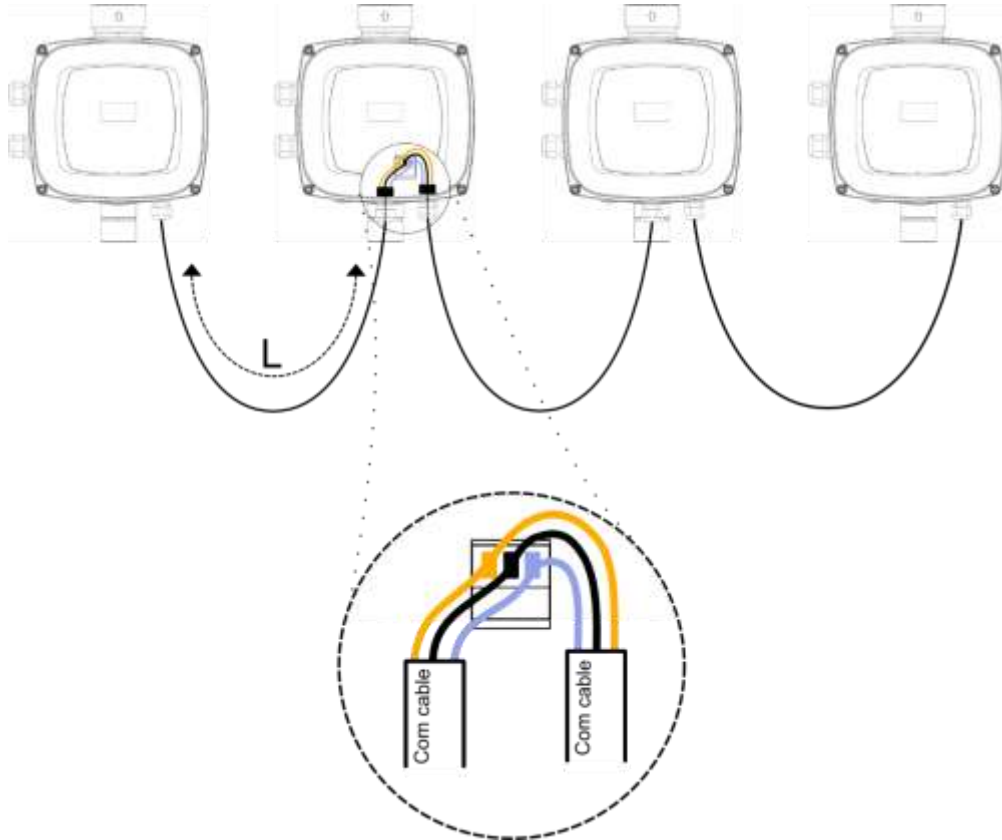
Figure 6: Example of connection of the multi-inverter communication with 4 devices
