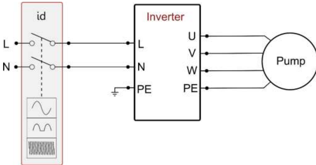
Figure 2a: Example of installation with single-phase power supply
