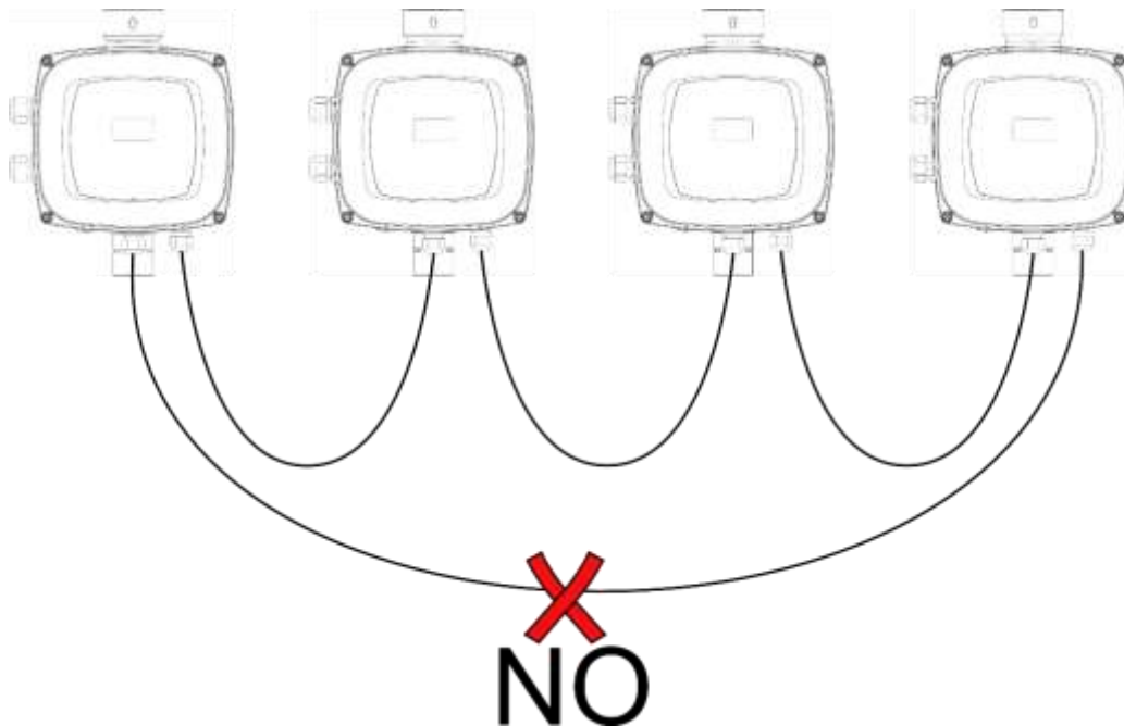
Figure 7: Do not make loop connections
