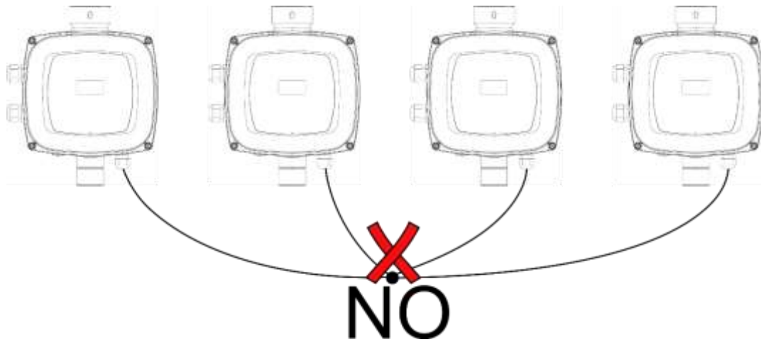
Figure 8: Do not make star connections
