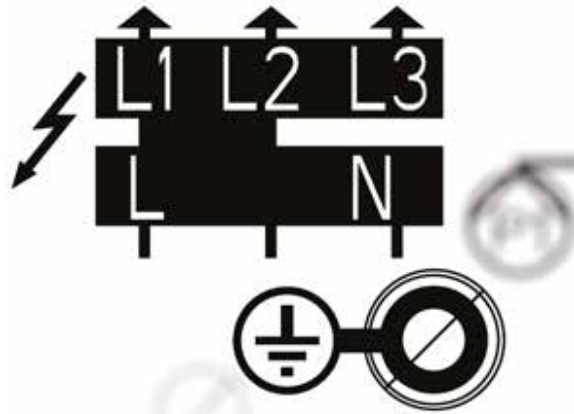
Figure 5: Electrical connection to the supply line
