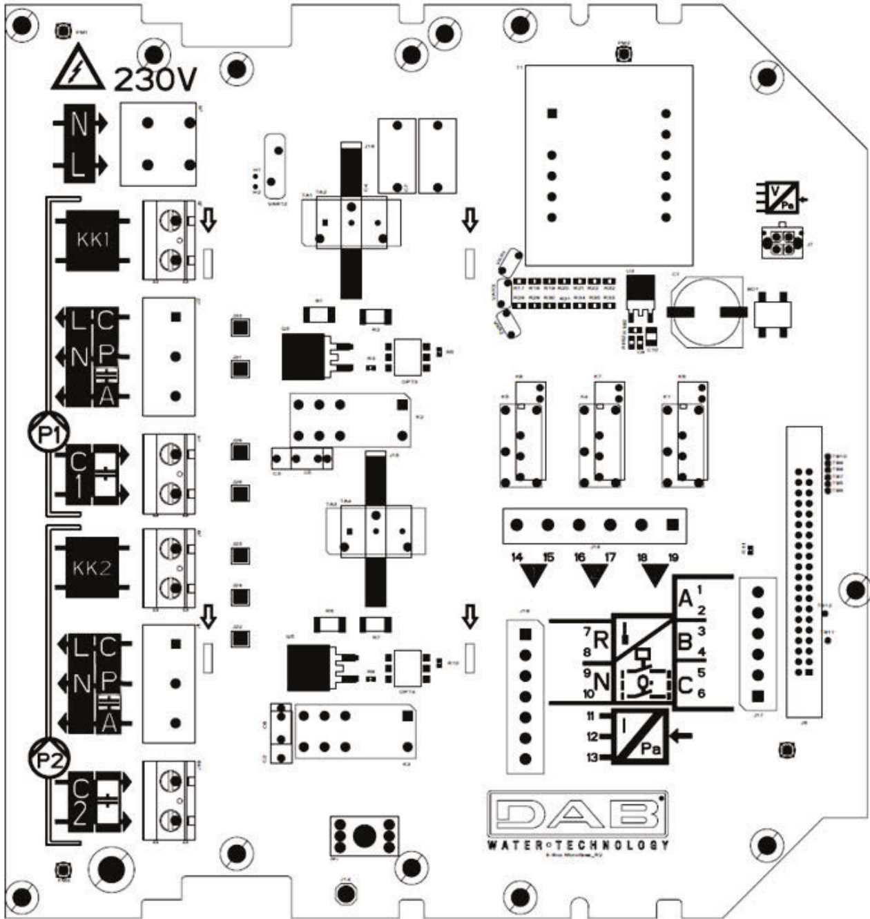
Figure 1: Ebox Basic Board
