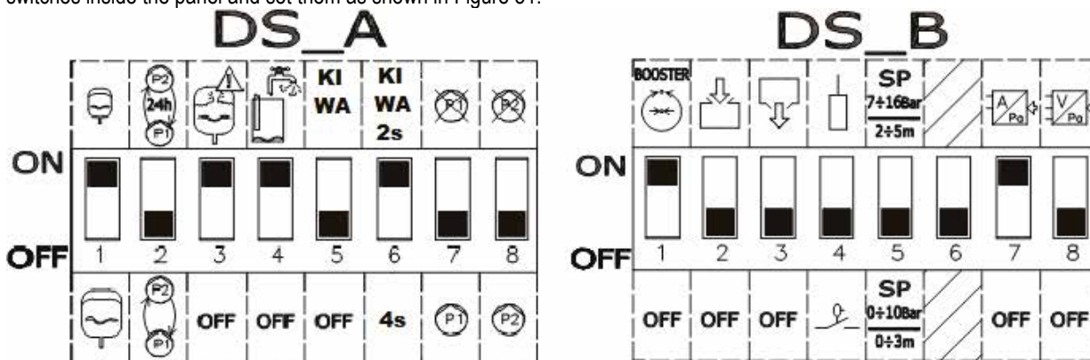
Figure 51: Dip switches for KIWA pressure boosting
