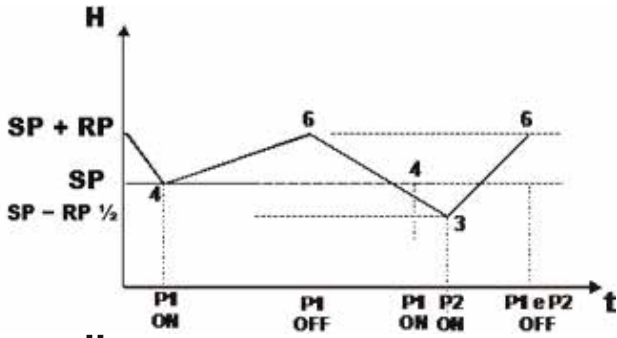
Figure 54: Regulation with expansion vessel < 100 litres
