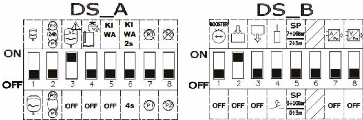
Figure 27: Setting the filling dip switches
