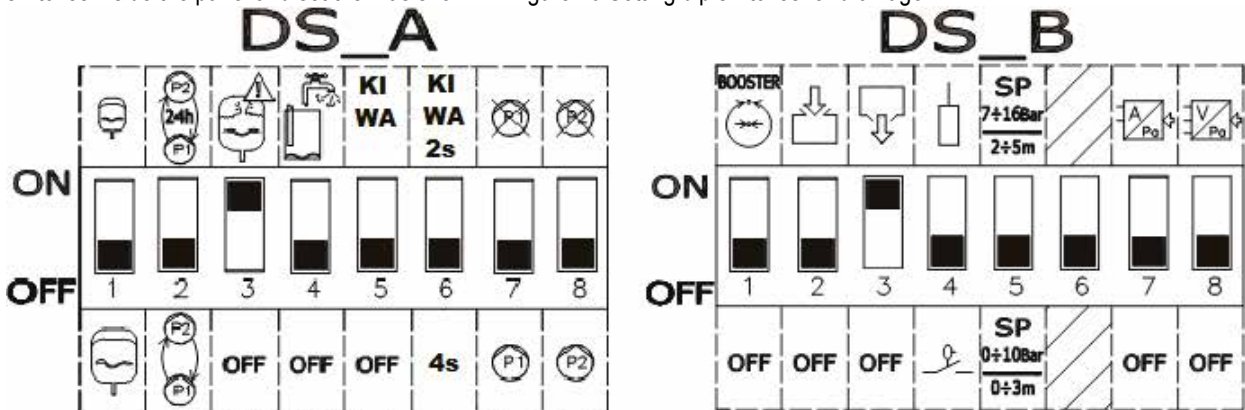
Figure 40: Setting the Drainage dip switches
