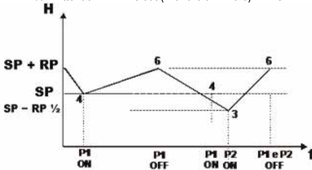
Figura 17: Regulation with expansion vessel < 100 litres
