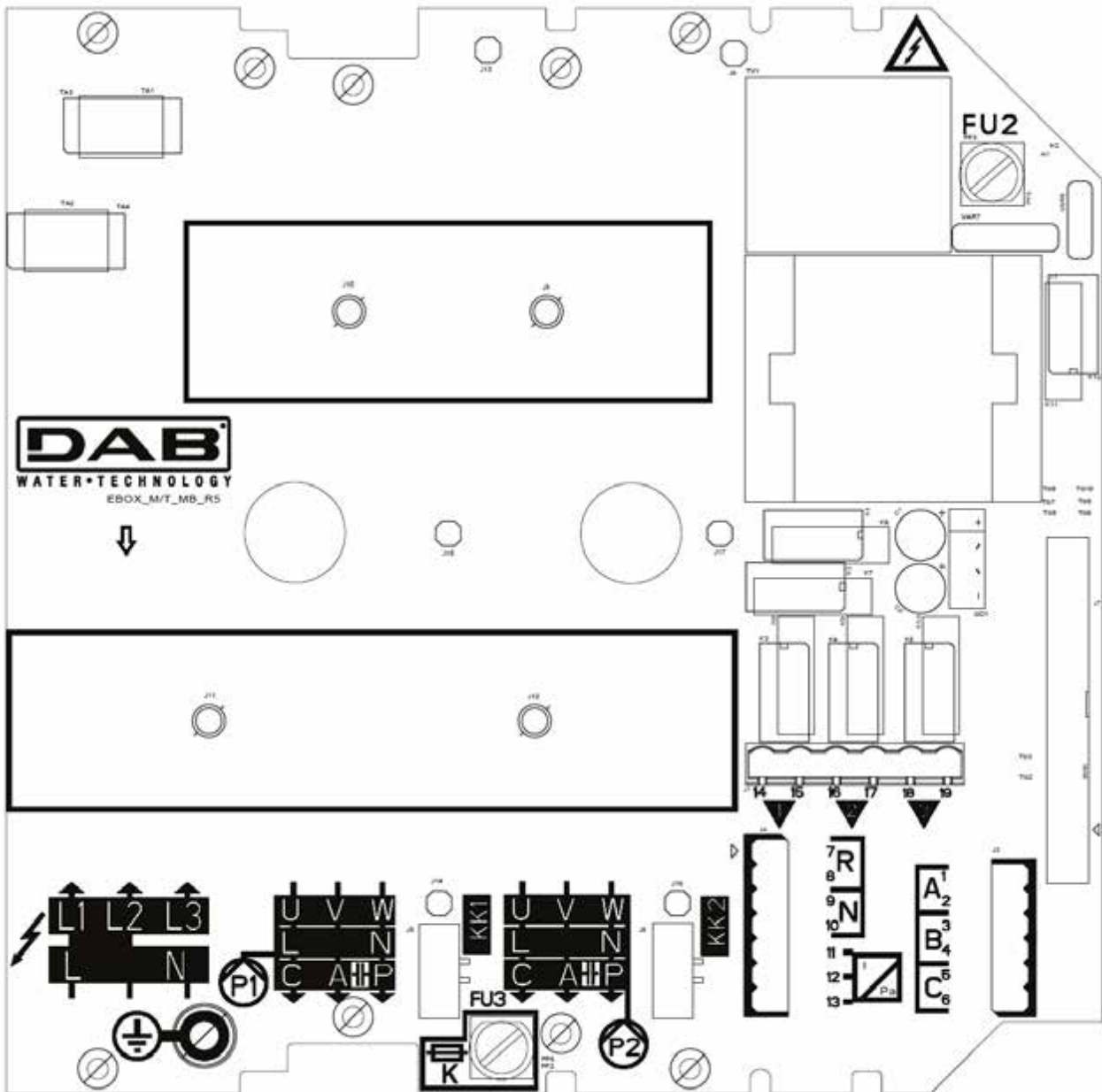
Figure 2: Ebox Plus Board
