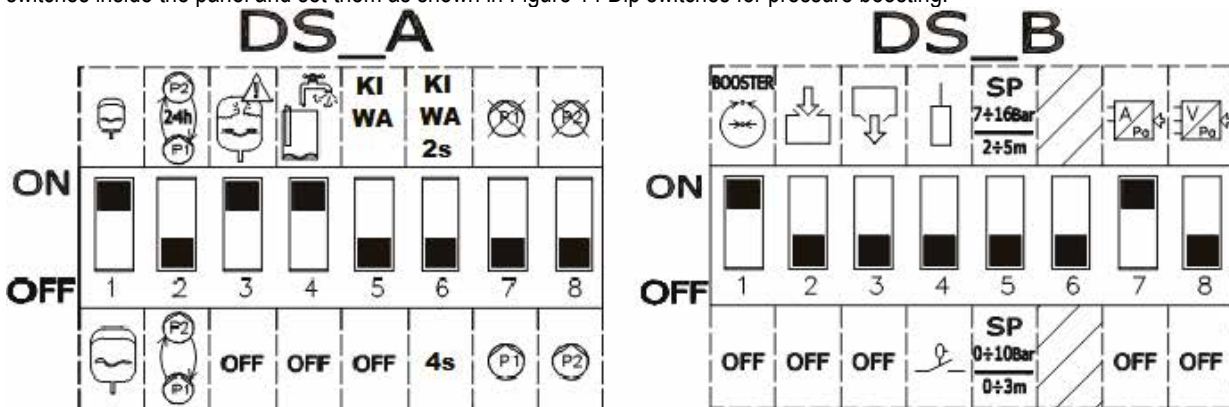
Figure 14: Dip switches for pressure boosting
