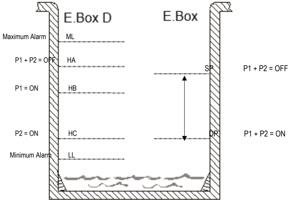
Figure 30: Filling with a depth sensor
