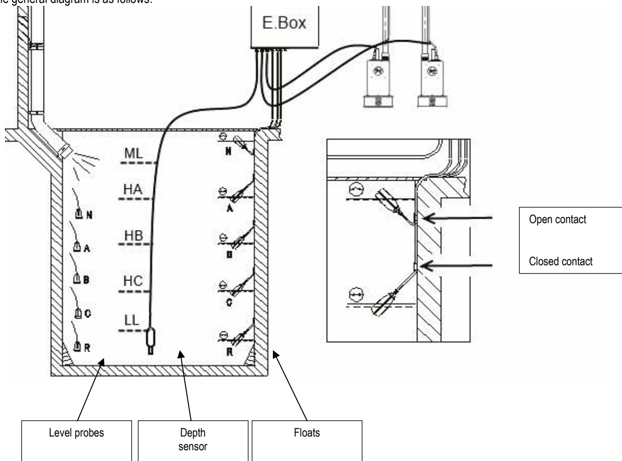
Figure 19: Diagram of filling system inputs
